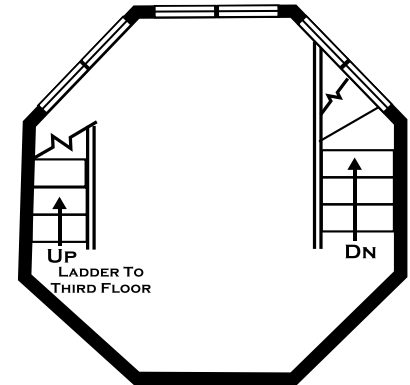
WATER TOWER SECOND FLOOR
