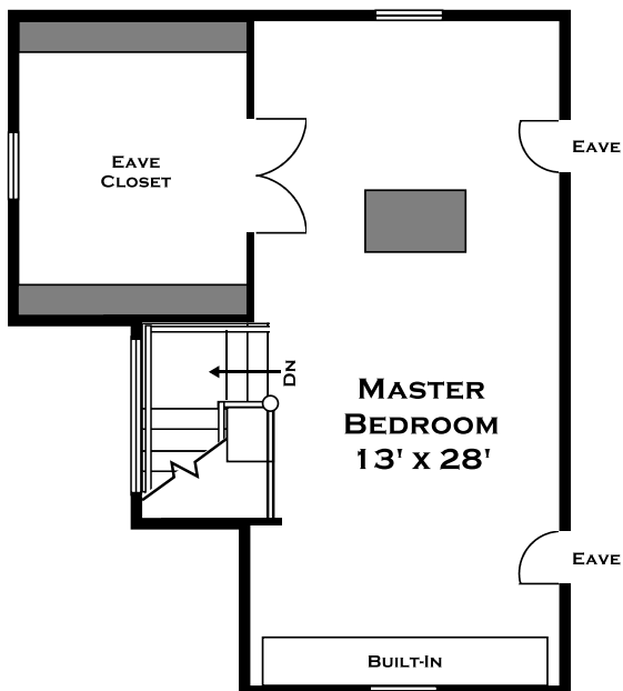
THIRD FLOOR
